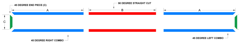
FRAME SECTION DETAIL
