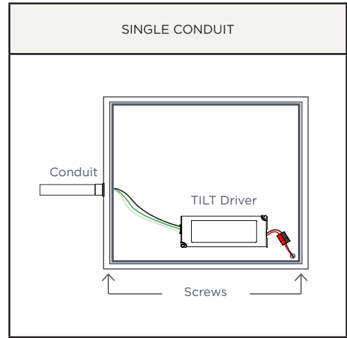
PASS THROUGH CONDUIT
